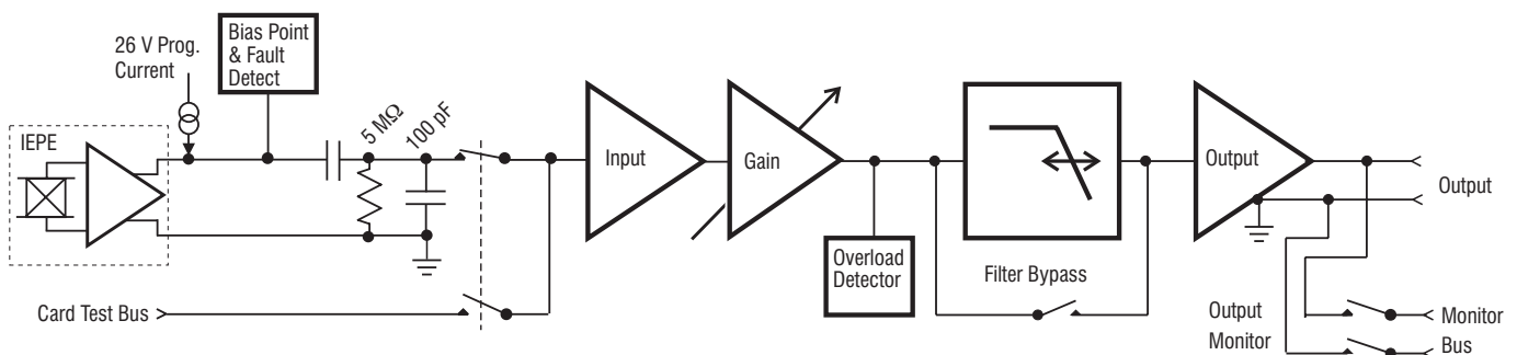
28316A Channel Block Diagram
