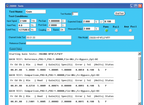
The FAT test screen reports the test conditions and provides a tabular listing of the test results during the execution of the test sequence.
