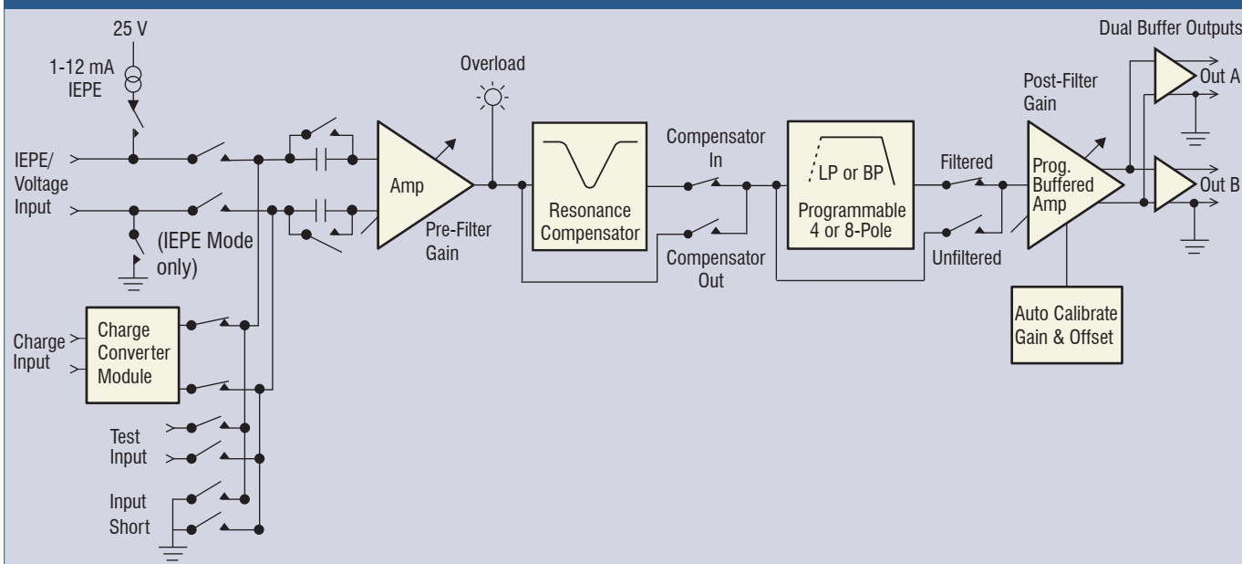
28304 Channel Simplified Block Diagram
