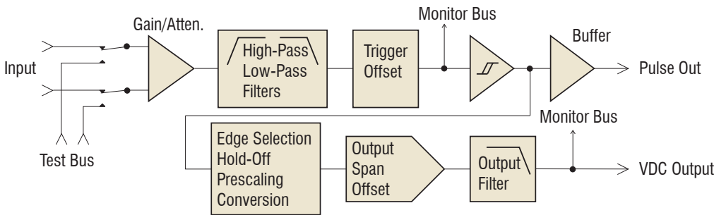
Block Diagram of Typical 28524 Channel
