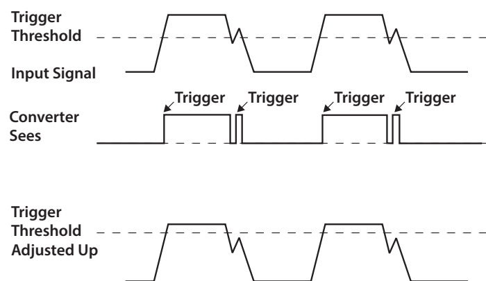
Figure 3 Programmable Trigger Threshold
